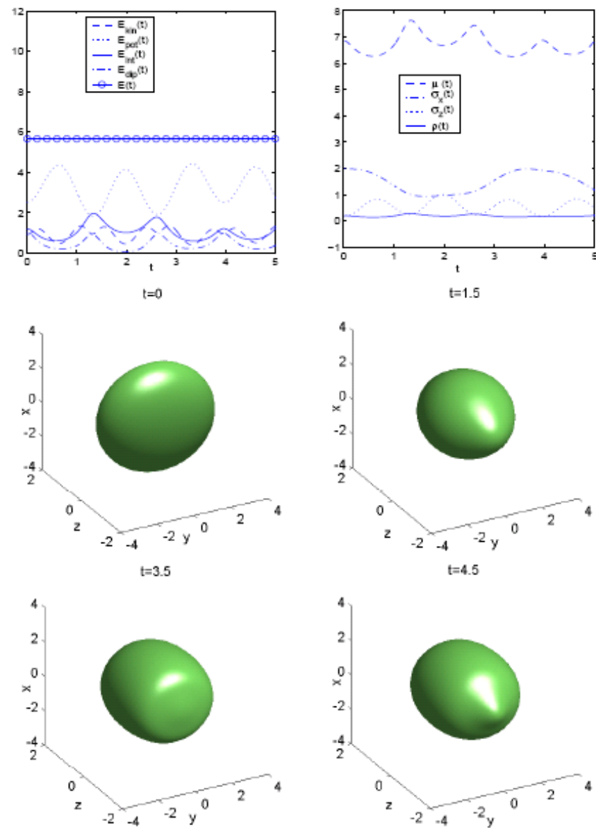
Figure 4: Time evolution of different quantities and isosurface plots of the density function \rho(\mathbf{x}, t) := |\psi(\mathbf{x}, t)|^2 = 0.01 at different times for a dipolar BEC when the trap potential is suddenly changed from \frac{1}{2}(x^2 + y^2 + 25z^2) to \frac{1}{2}(x^2 + y^2 + \frac{25}{4}z^2) at time t = 0 .
