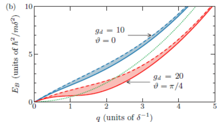
FIG. 6. (Color online) Bogoliubov energies for different polarizations and DDI strengths. (a) Polar plots marked with the magnitude and angle of \mathbf{q} . White areas mark unstable regions. (b) Cuts through Bogoliubov energies at the polar angles indicated in (a). Solid lines include intra- and interlayer DDIs, whereas dashed lines only include the intralayer DDI. The green dotted line represents ^{52}\text{Cr} . The interlayer DDI does not influence high energies where the in-plane excitations become particle-like. Parameters are as in Fig. 3, with g = 0 and \nu = 1/10 .
