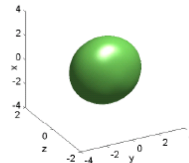
Figure 3: Time evolution of different quantities and isosurface plots of the density function \rho(\mathbf{x}, t) := |\psi(\mathbf{x}, t)|^2 = 0.01 at different times for a dipolar BEC when the dipolar direction is suddenly changed from \mathbf{n} = (0, 0, 1)^T to (1, 0, 0)^T at time t = 0 .
